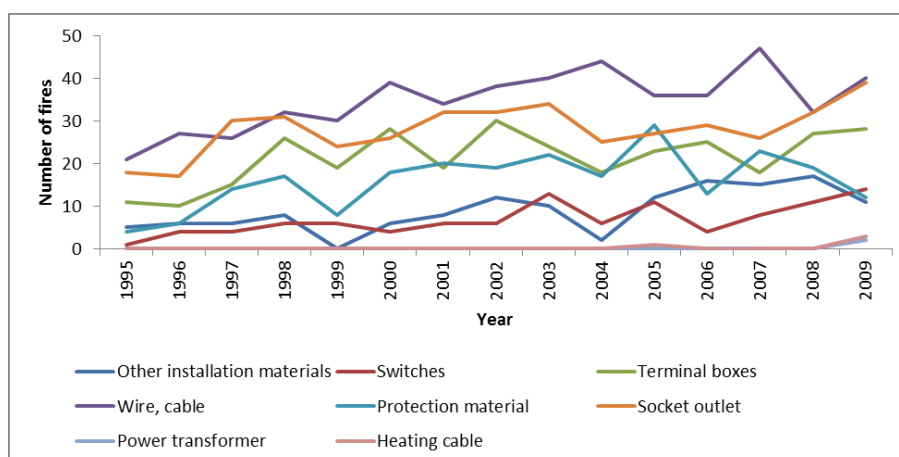
Figure 3-4 Distribution of the number of residential fires according to the type of installation materials causing the fire, in the period 1995-2009 (the figure is based on data from the DSB fire statistics).
